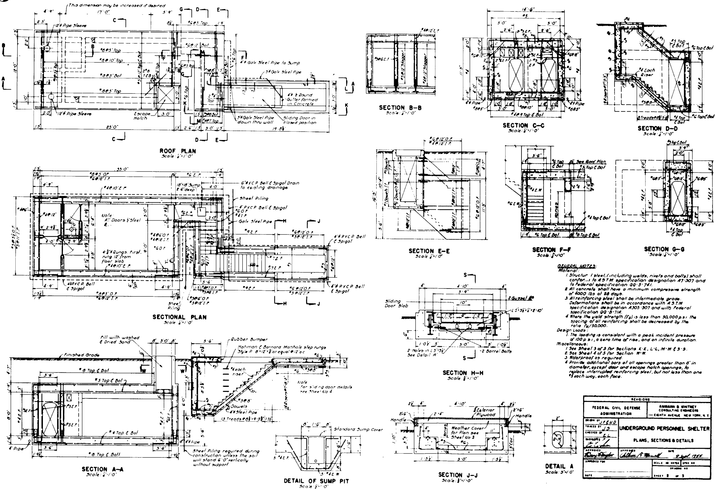
Fig. 16—Plans, sections, and details, underground personnel shelter.
